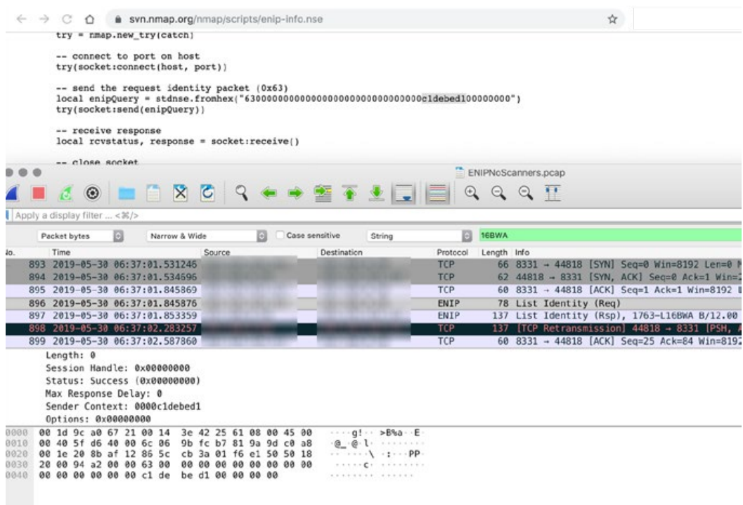
Figure 59. Comparing the Allen-Bradley MicroLogix 1100 PLC traffic to enip-info.nse, where the sender context is the same
