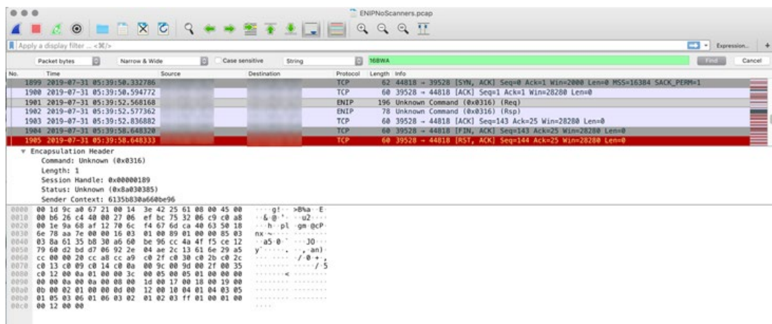
Figure 60. An unknown command sent to the Allen-Bradley MicroLogix 1100 PLC
